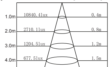
Lux distance Curve [Unit: Lux]
